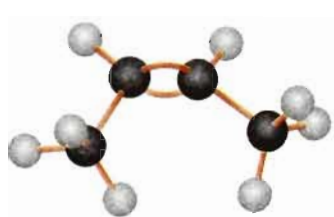
a) cis -but-2-en t_{nc} = -139^\circ\text{C} t_s = 4^\circ\text{C}
