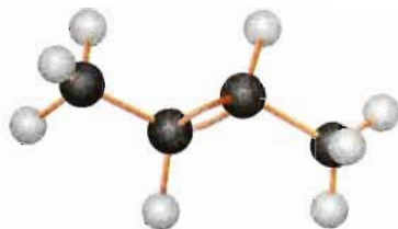
b) trans -but-2-en t_{nc} = -106^\circ\text{C} t_s = 1^\circ\text{C}
